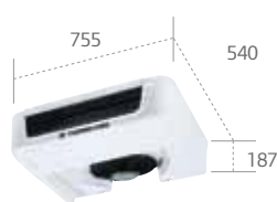
ES150 Ultra slim evaporator
