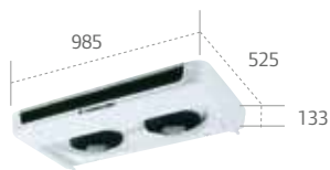
ES200 Ultra slim evaporator
